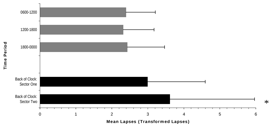
Figure 13: PVT transformed lapses
