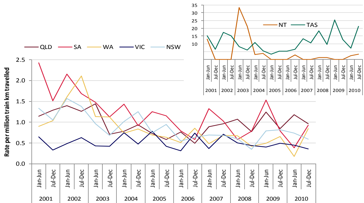
Figure 1: Normalised biannual rate of Australian running line derailments per million km travelled by jurisdiction and year, 1 January 2001 to 31 December 2010
