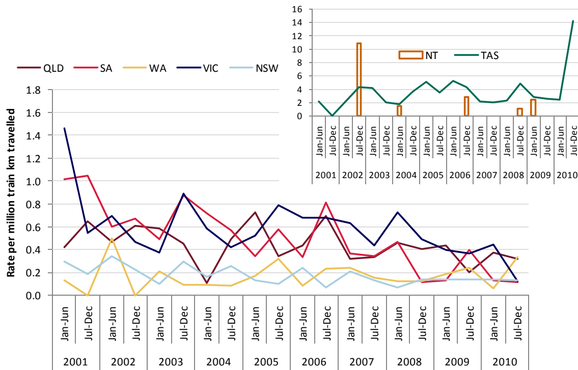
Figure 5: Normalised road vehicle collisions at level crossings, biannual rate per million train km travelled by jurisdiction and year, 1 January 2001 to 31 December 2010
