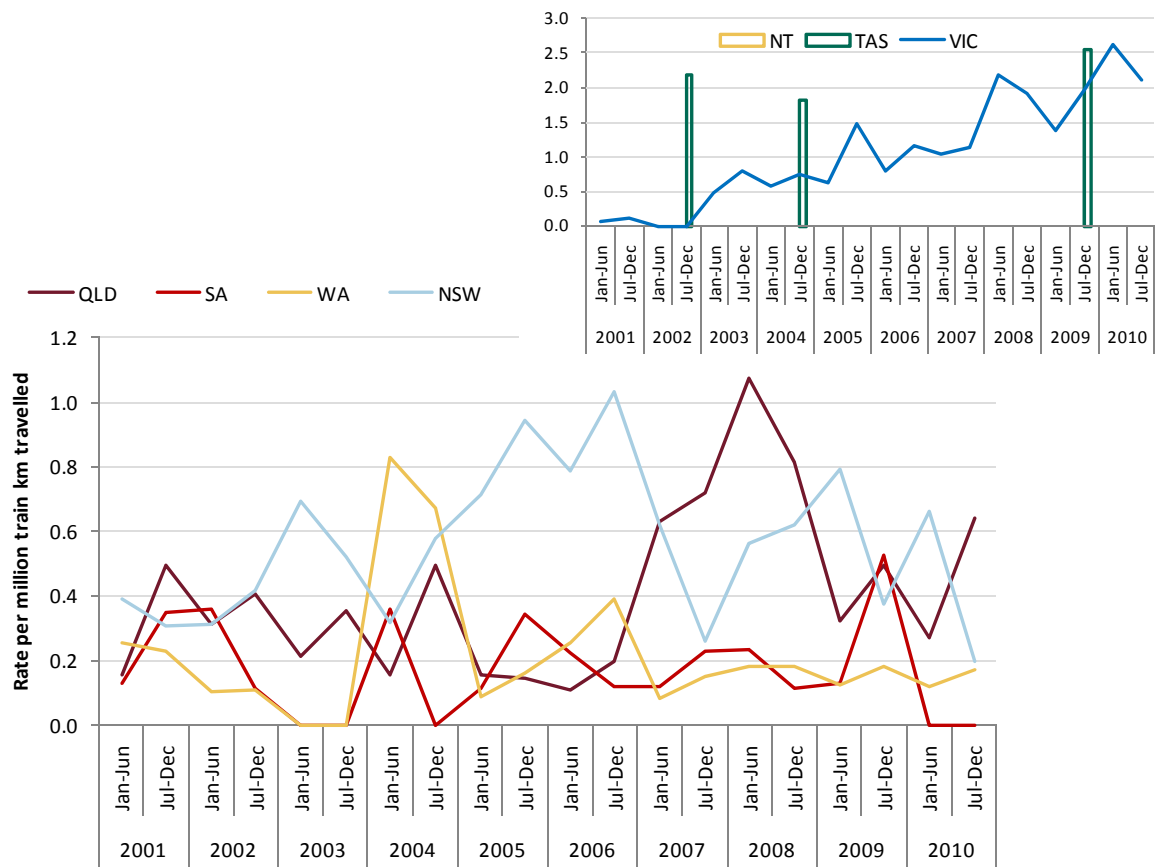
Figure 3: Normalised running line collisions with infrastructure, biannual rate per million train km travelled by jurisdiction and year, 1 January 2001 to 31 December 2010
