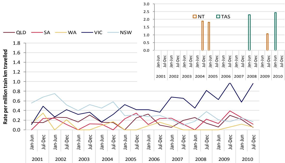
Figure 2: Normalised running line collisions with person (not at a level crossing), biannual rate per million train km travelled by jurisdiction and year, 1 January 2001 to 31 December 2010
