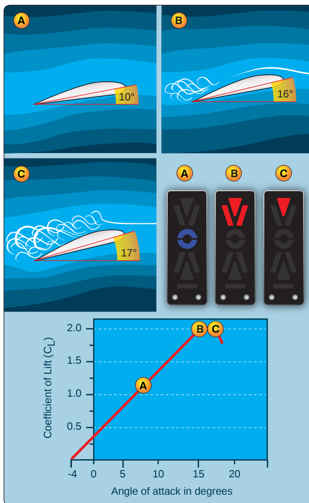
Figure 4-5. A conceptual representation of an AOA indicator. It is important to become familiar with the equipment installed in a specific airplane.
