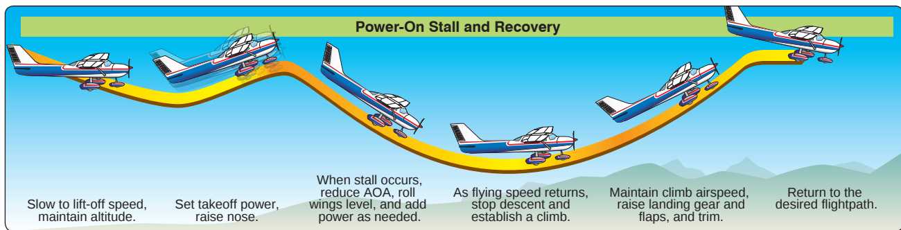
Figure 4-8. Power-on stall.
