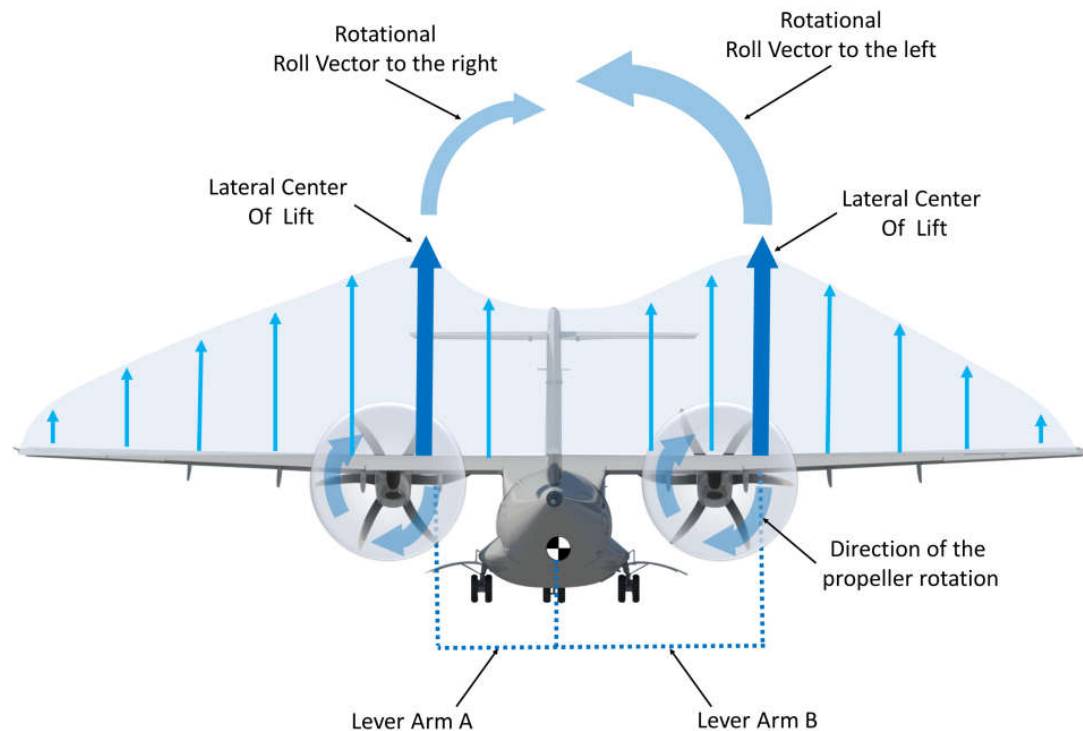
Accelerated slipstream – roll moment
