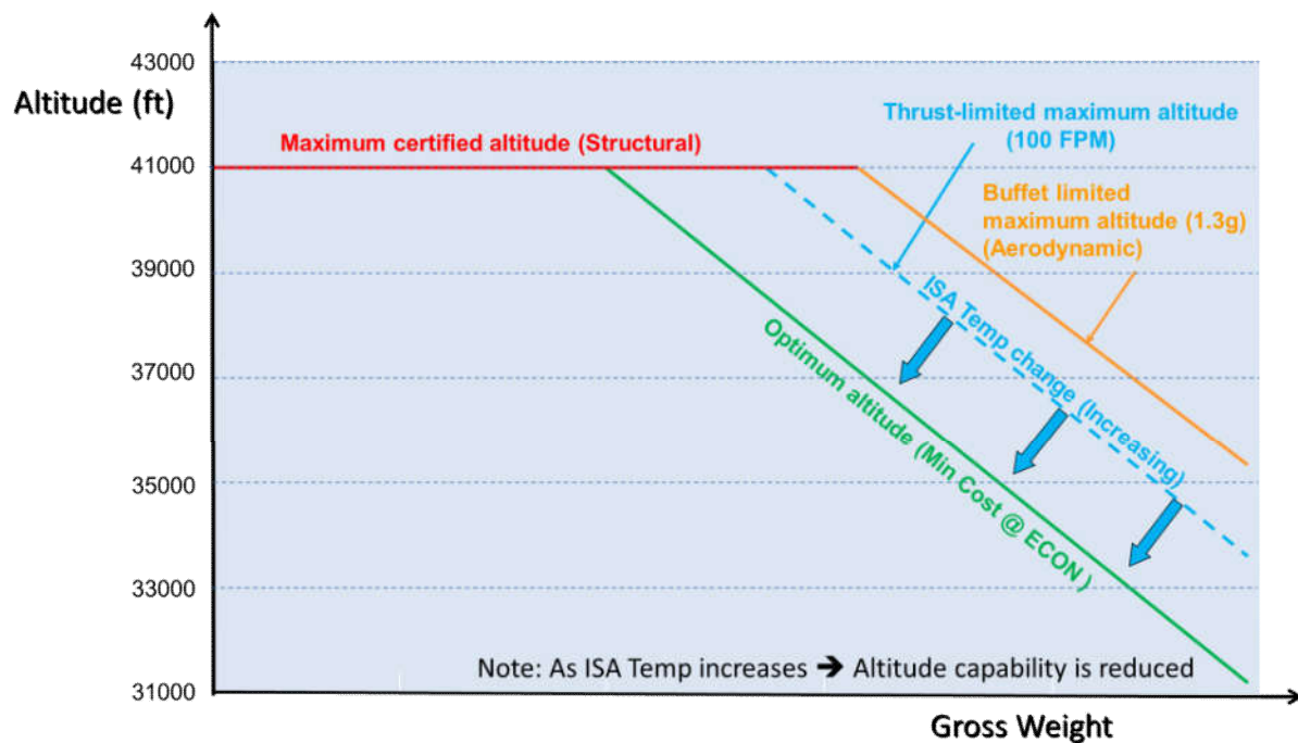
Typical Optimum Altitude vs. Maximum Altitude
