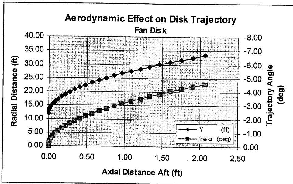
FIGURE 4-10. HBR FAN DISK WINDAGE EFFECTS
