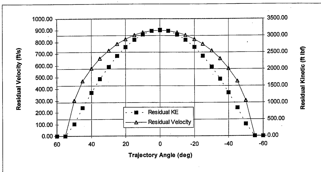
FIGURE A-3. INITIAL DEBRIS ENERGY VERSUS TRAJECTORY ANGLE
